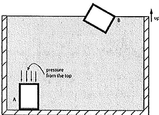
Fig. 2. An example where Archimedes law is violated. In situation A, a buoyant barrel with a perfectly flat bottom (say, glass) is placed near the bottom of a container that also has a perfectly flat bottom. No water can get under the barrel so the barrel does not float even though it displaces more water than its own weight (see text). However, once water does get under the barrel, the barrel does float (situation B).
